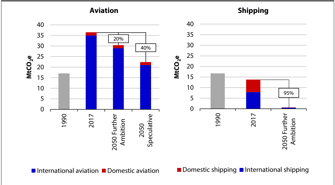
Figure A7. Aviation and shipping emission scenarios to 2050
